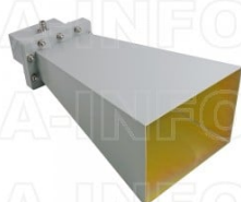
LB-510-10-C-NF Standard Gain Horn Antenna 1.45-2.2GHz 10dB Gain N Type Female
