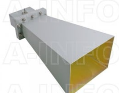
LB-510-10-C-SF Standard Gain Horn Antenna 1.45-2.2GHz 10dB Gain SMA Female
